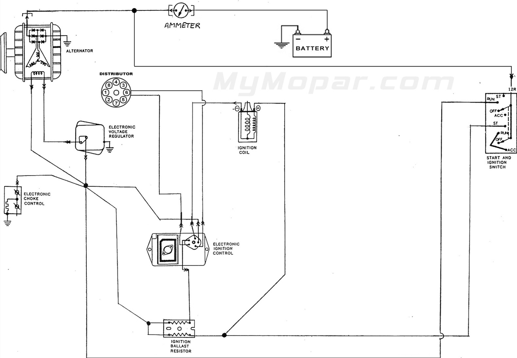
Chrysler Simplified Ignition & Charging Wiring Diagram Dual Ballast Resistor & 5-pin Electronic Ignition
